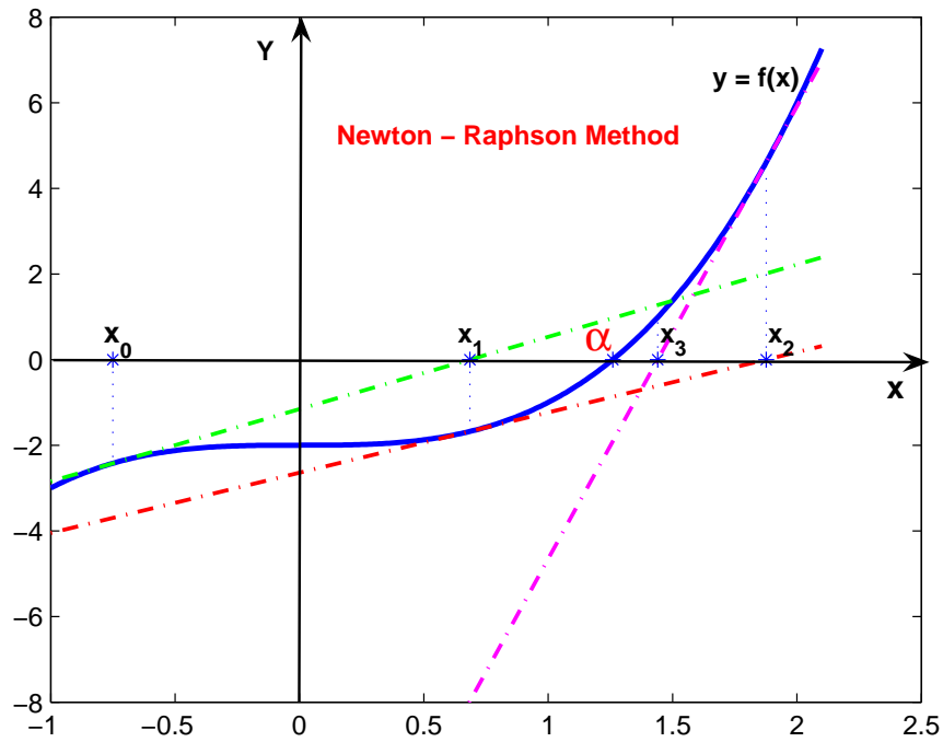
Figure 3: The Newton-Raphson method.
